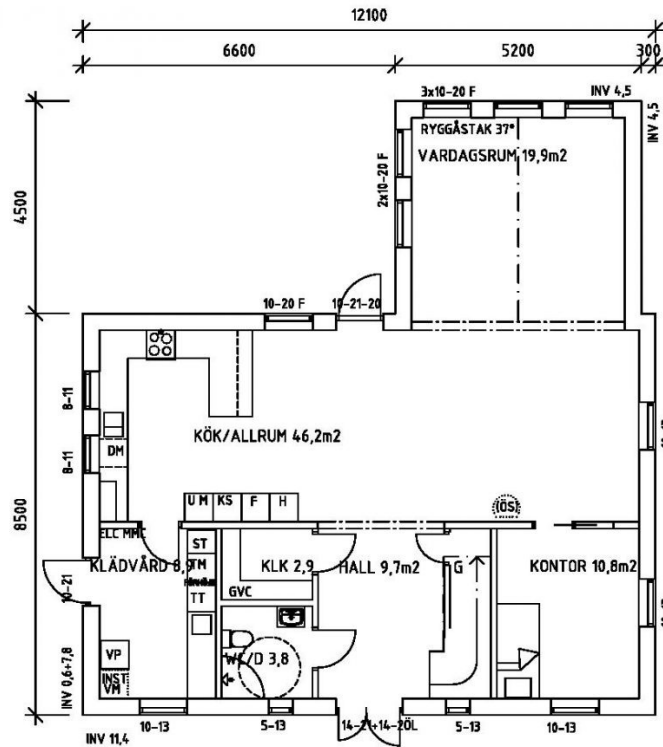
BOTTENPLAN 109,2m 2 BOA, 126,2m 2 BYA 185,1m 2 , 179,0m 2 BOA
