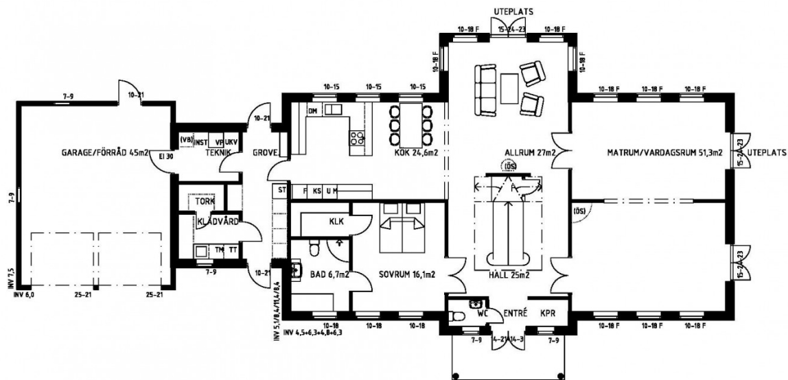
BOTTENPLAN 183,5m 2
