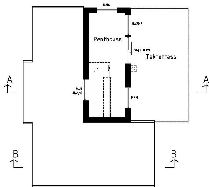
Takplan Inv. area: 16,6 m 2
