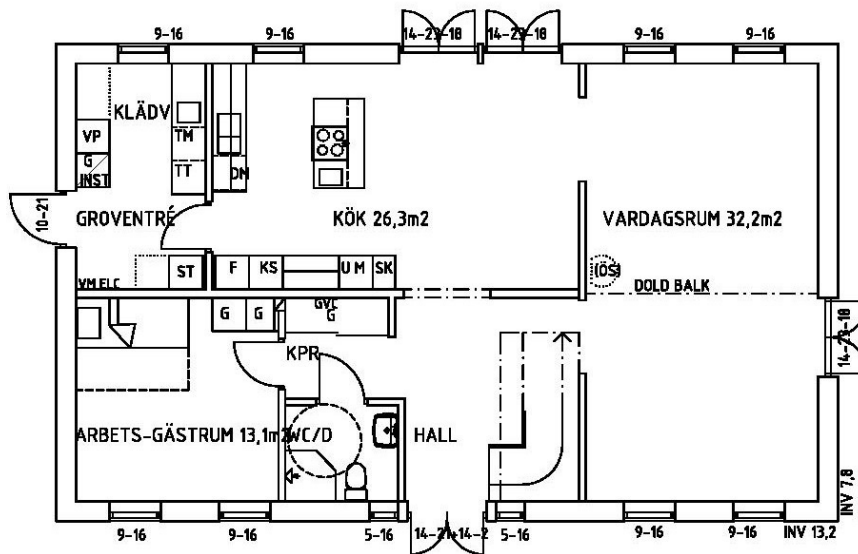
BOTTENPLAN, 103 m 2 BOAREA, 118m 2 BYA
