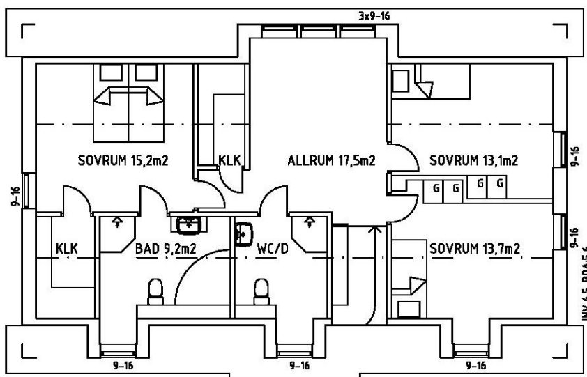
VINDSPLAN, 90,0m 2 Atemp, 80,9m 2 BOAREA
