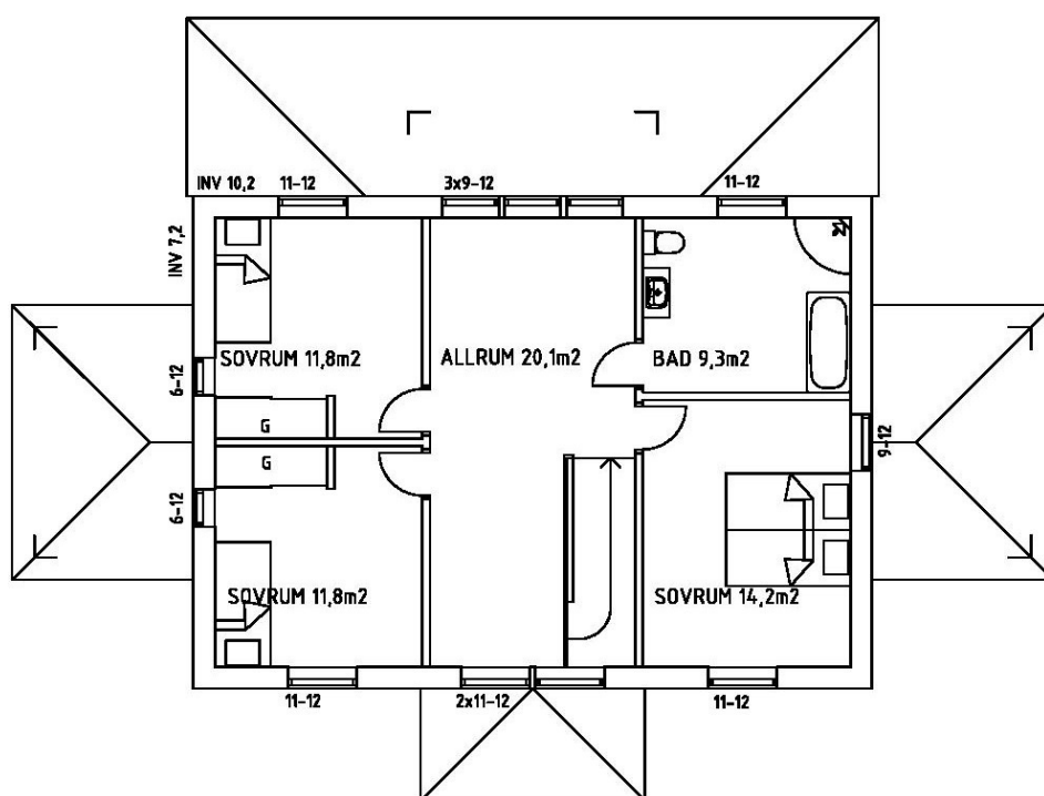
OVANPLAN 73,4m 2
