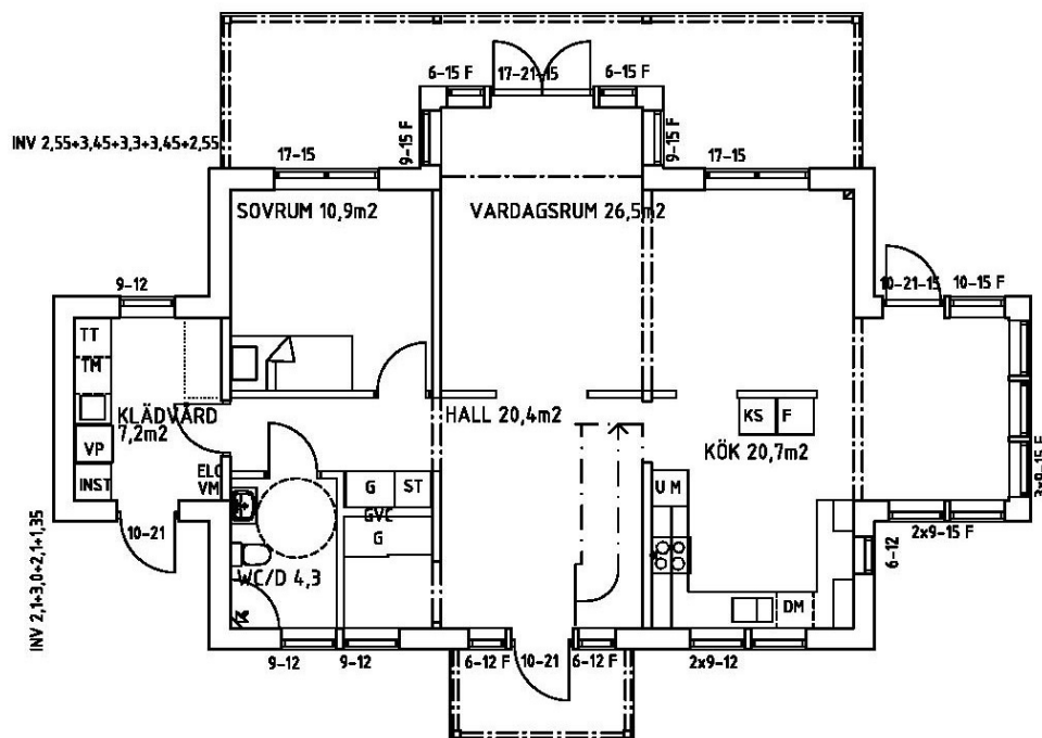
BOTTENPLAN 93,2m 2
