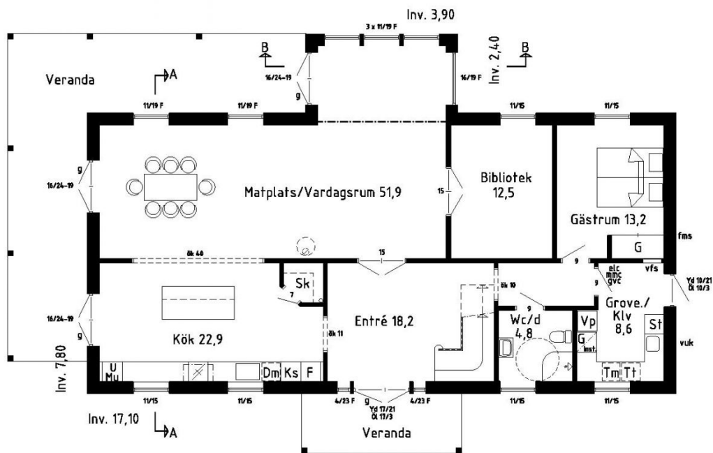
Bottenplan
